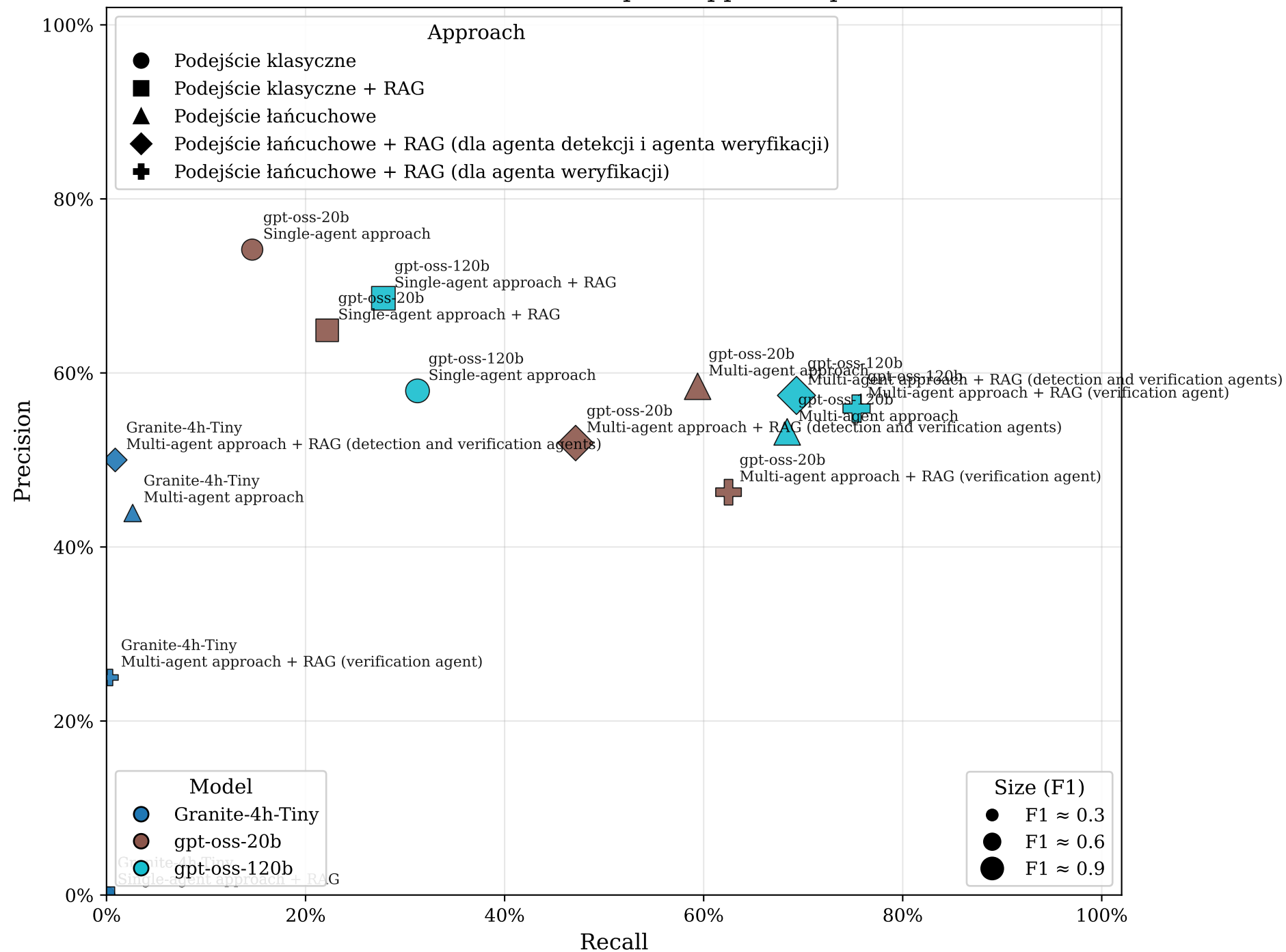
Precision-Recall relationship for vulnerability detection Point color = model, marker shape = approach, point size = F1
