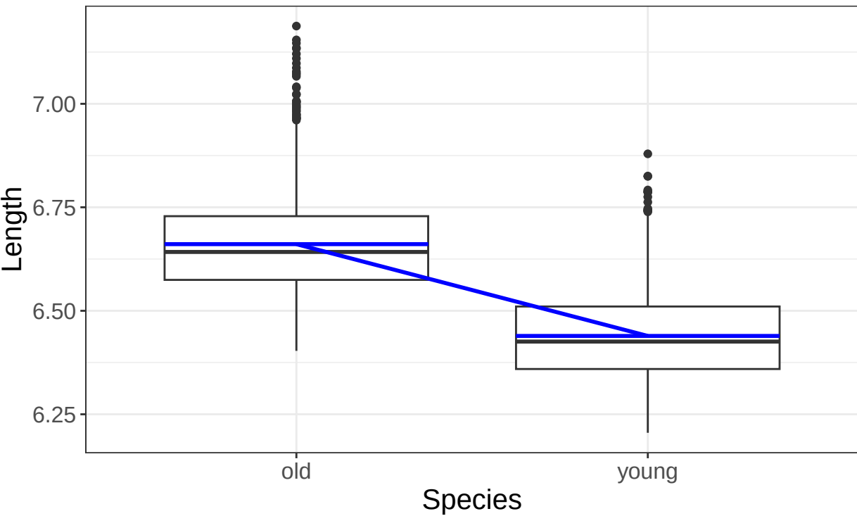
Boxplot raw data, predicted means (in blue) and trend with ggplot2
