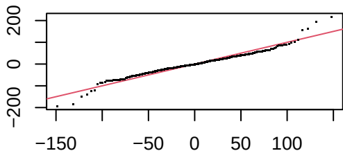
theoretical quantiles
