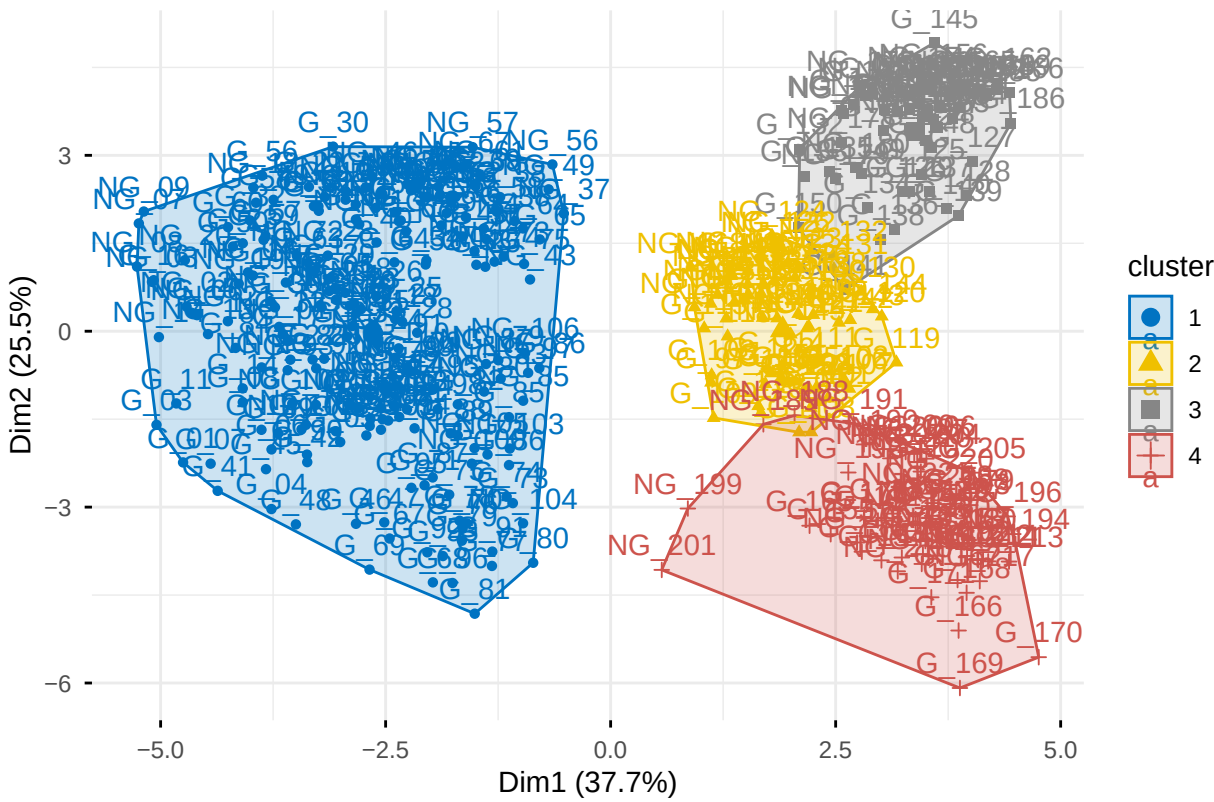
Cluster plot – 4 clusters
