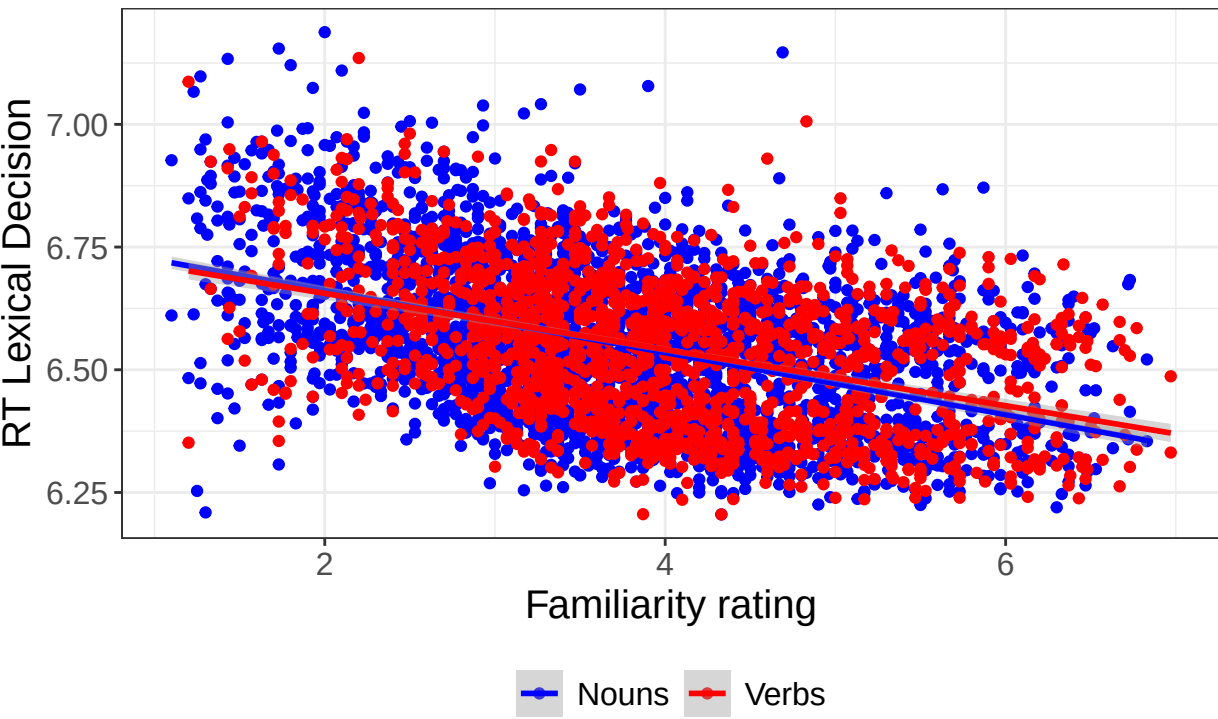
Familiarity rating vs RT in a lexical decision task with a trend line
