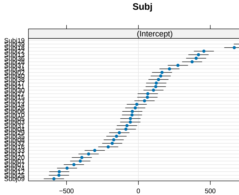
3.3.4.3.3.1 Subject Intercepts
