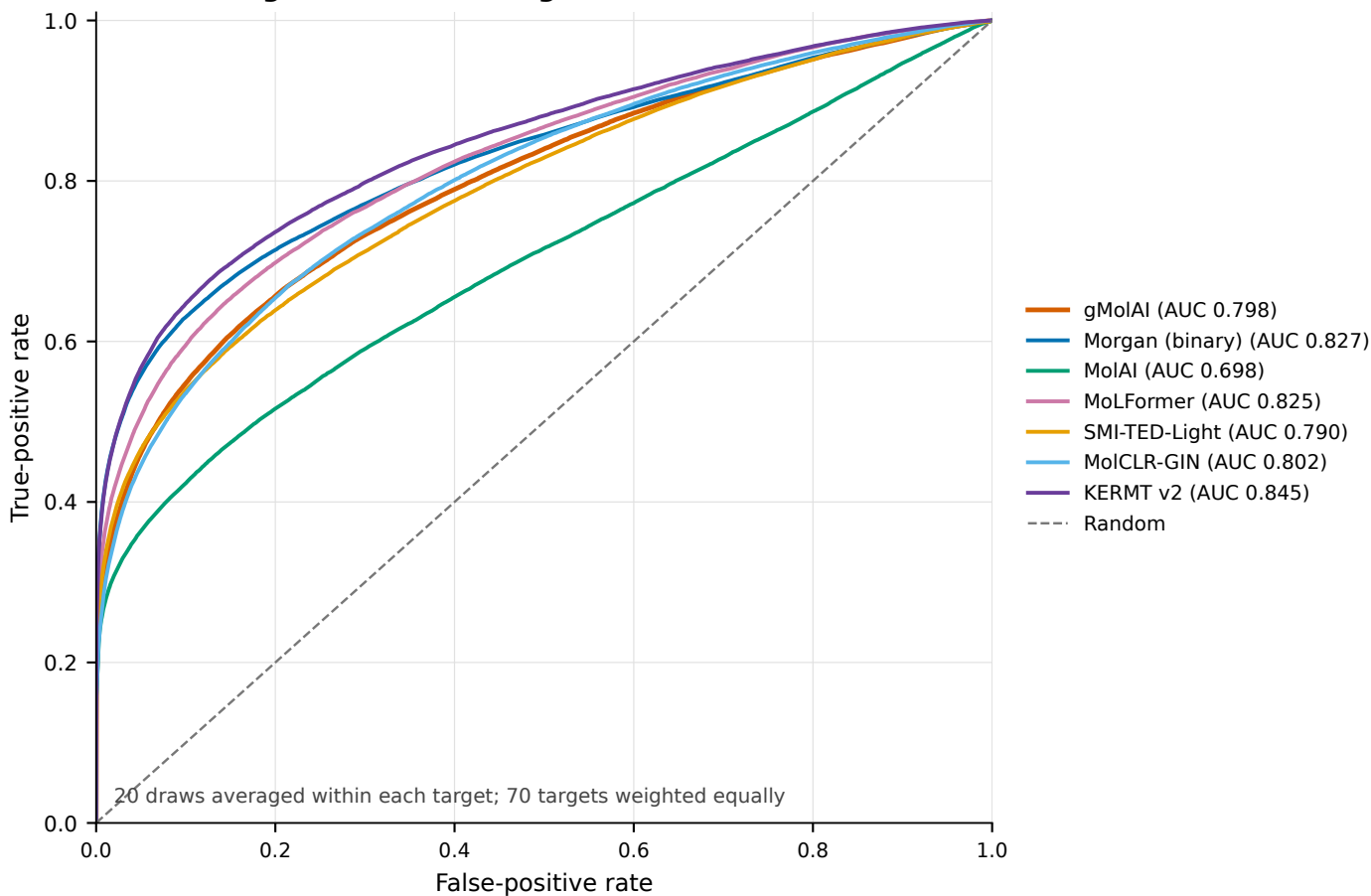
Five-shot ligand retrieval: target-balanced macro ROC
