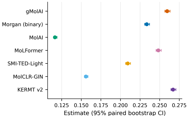
Normalized mutual information
