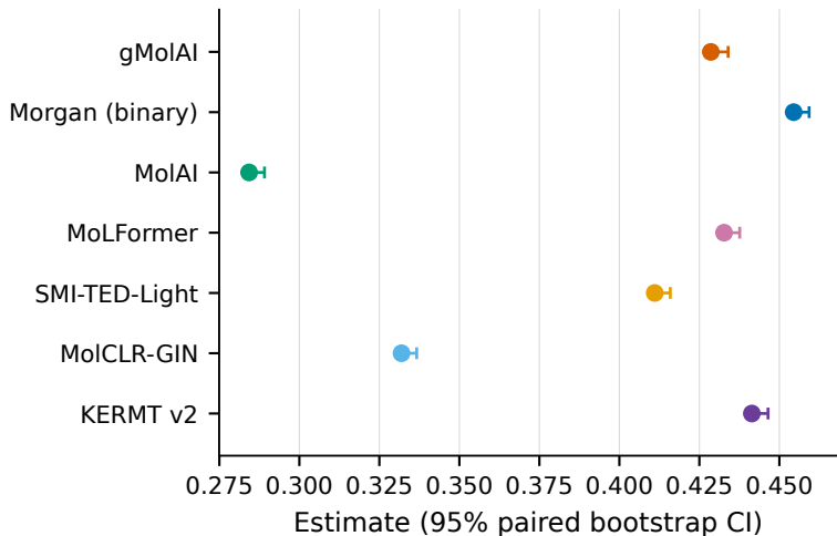
Normalized mutual information
