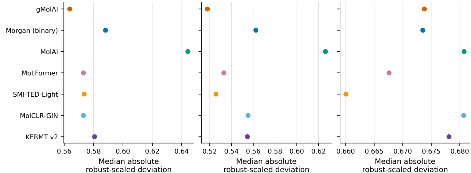
HOMO energy
