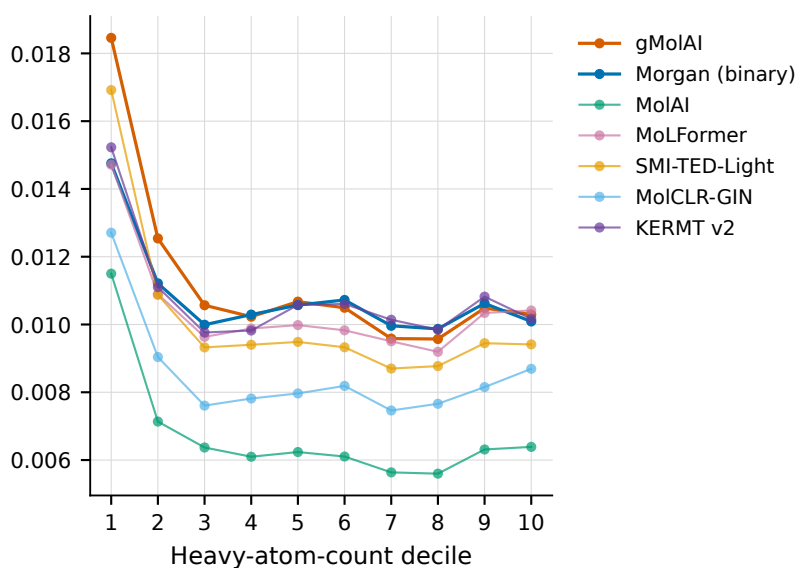
Property Recall@100
