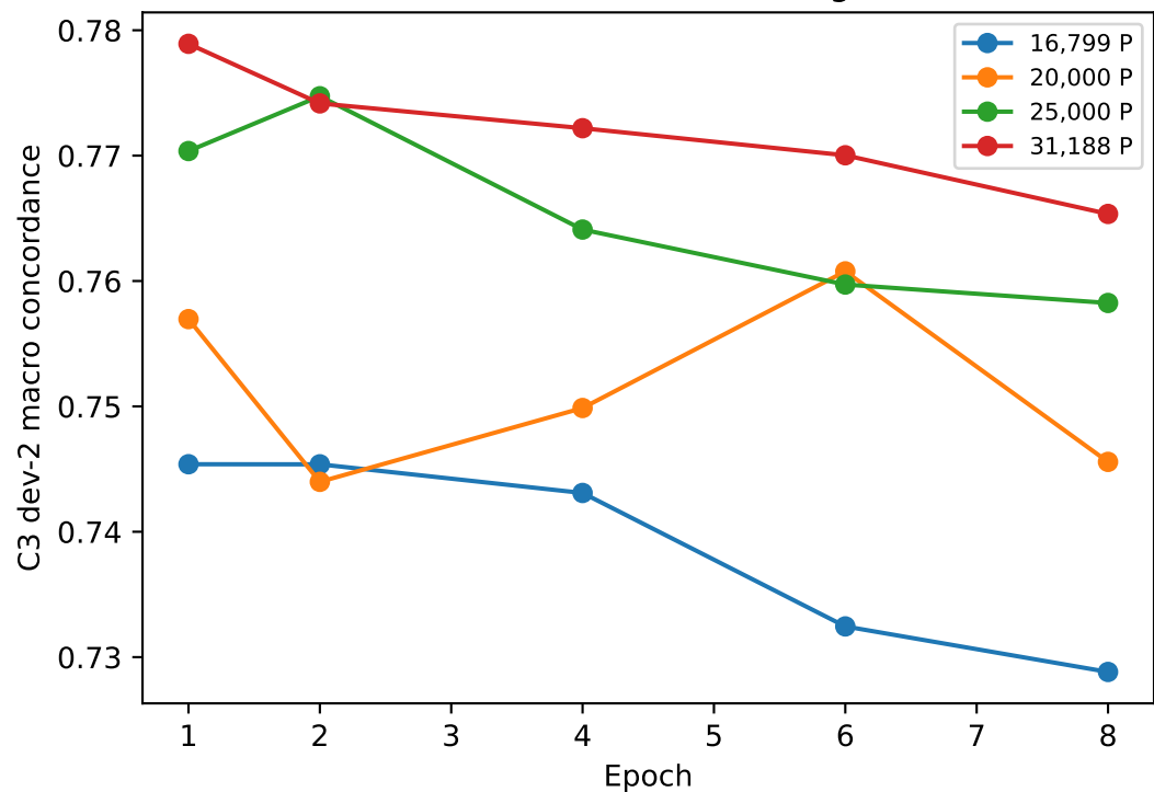
Three-seed ensemble learning curves
