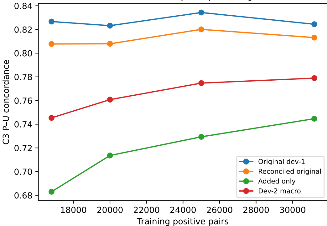
Best common epoch per budget
