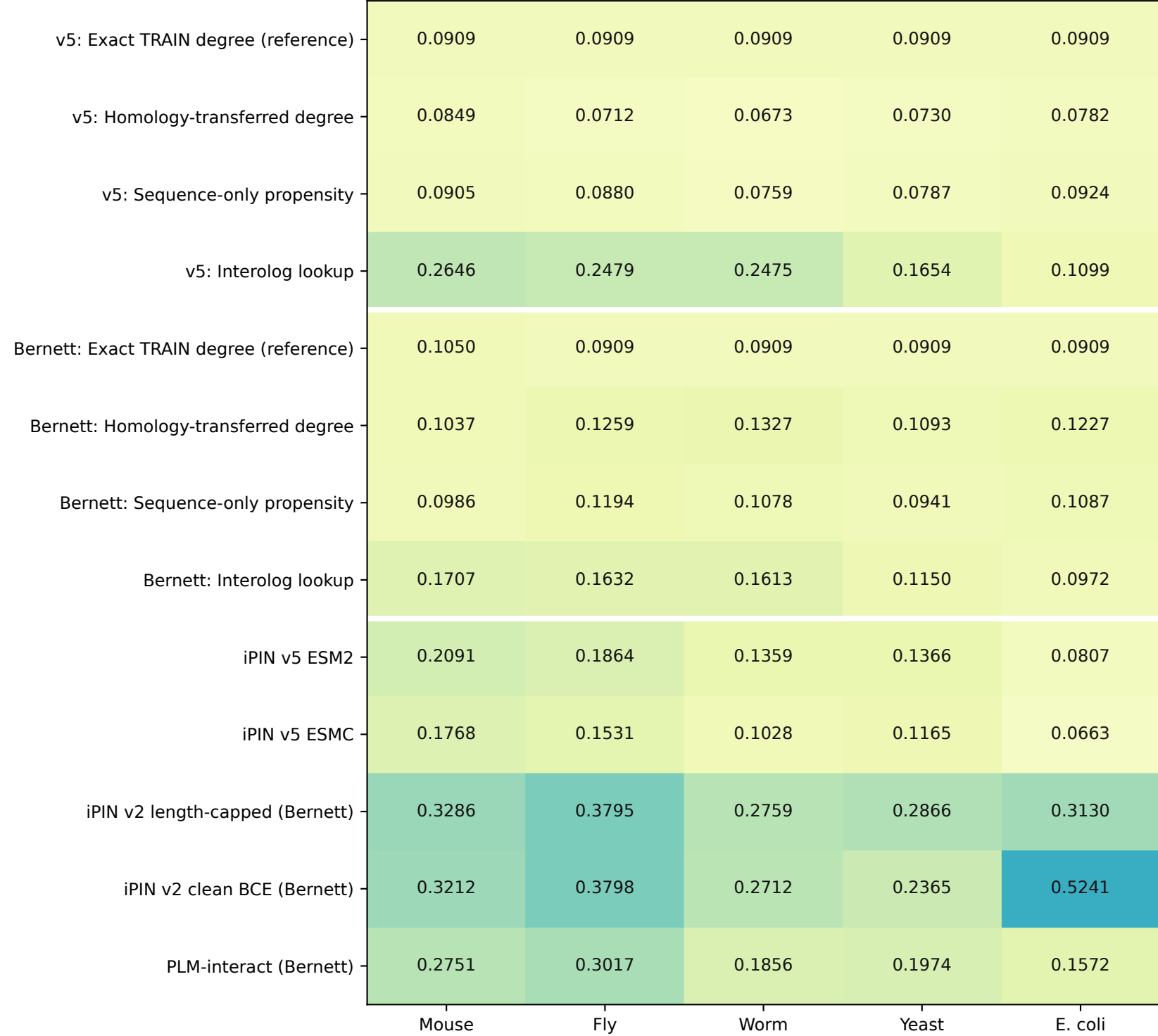
Five-species test | AP
