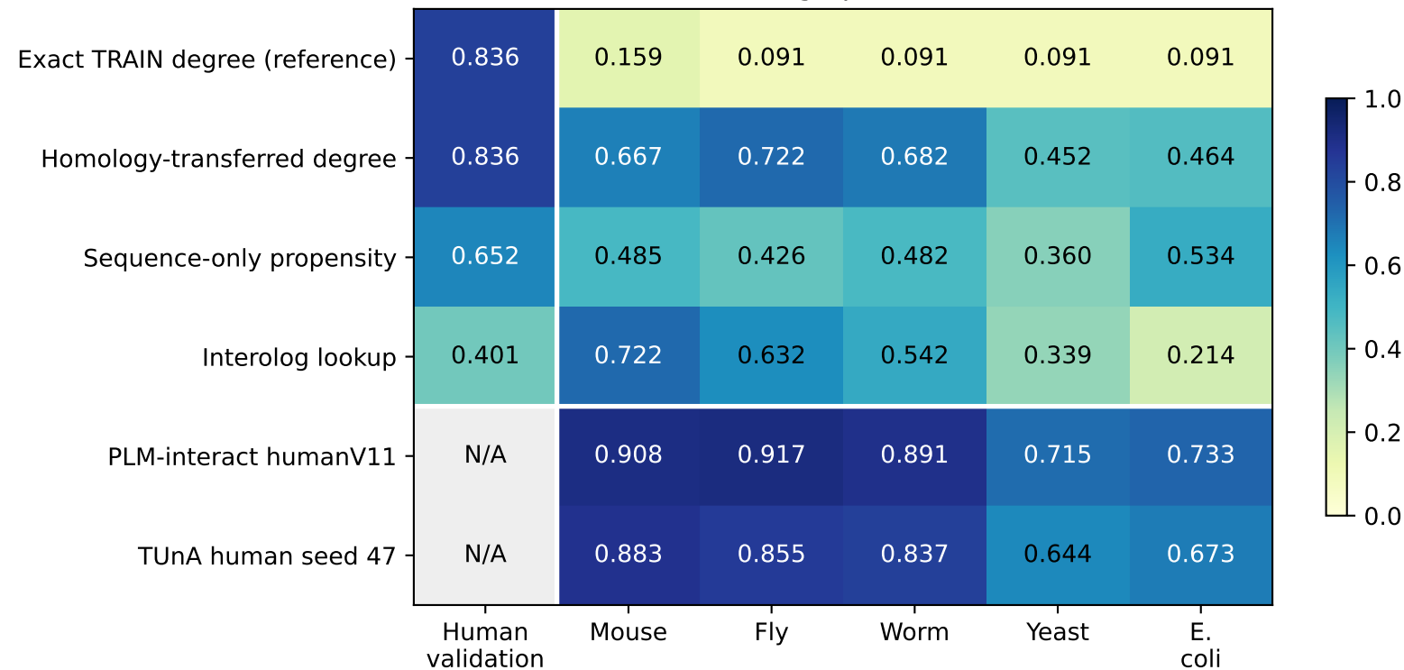
Average precision
