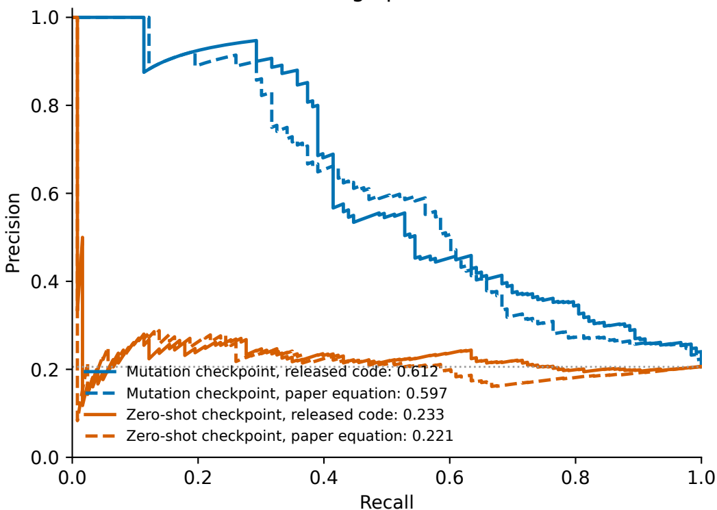
Average precision
