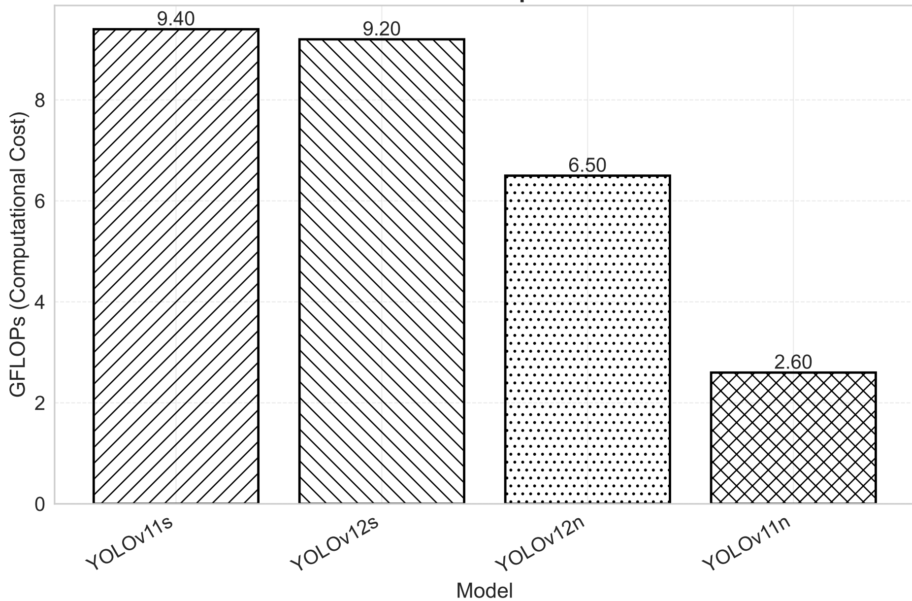
GFLOPs Comparison
