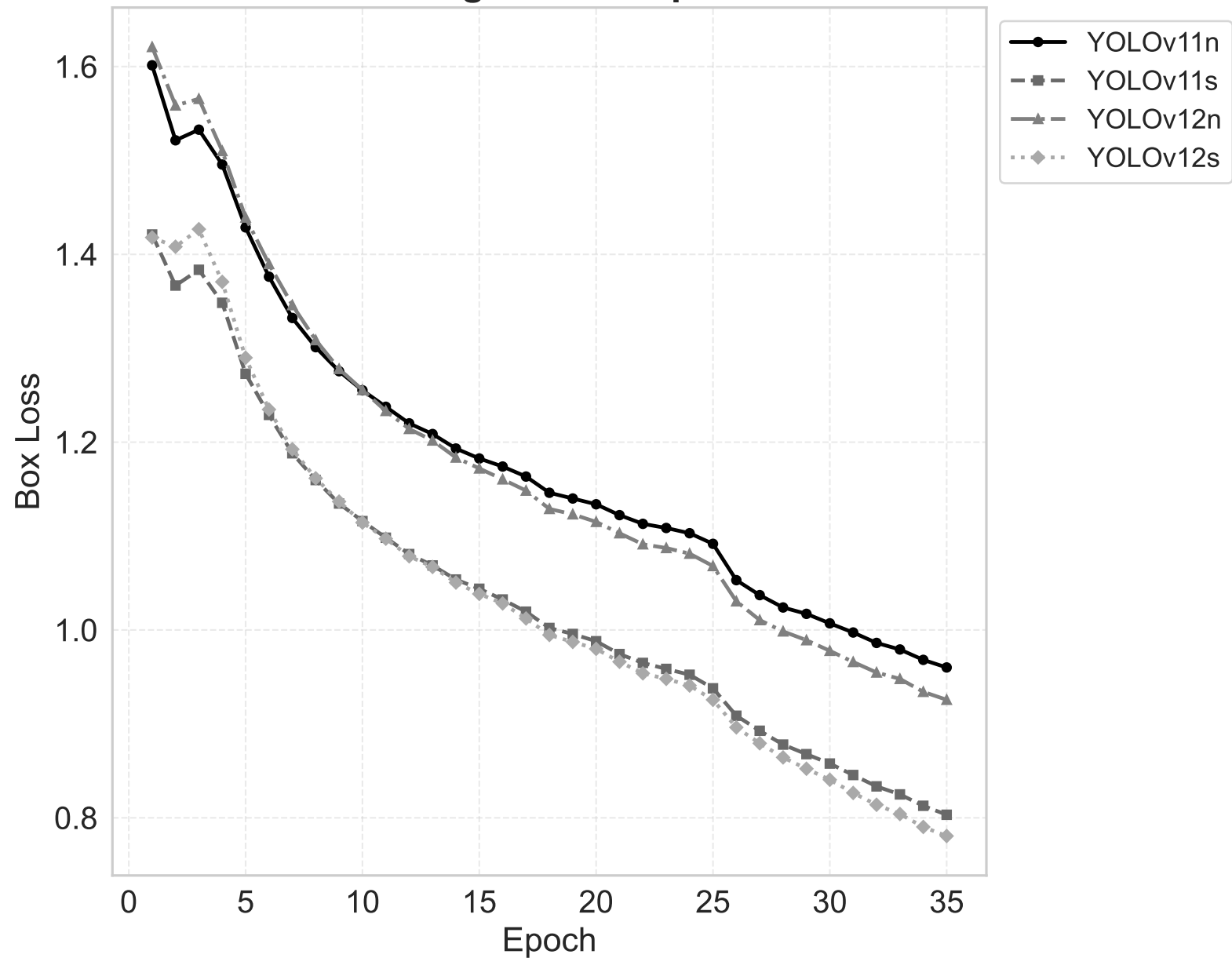
Training Loss vs Epoch
