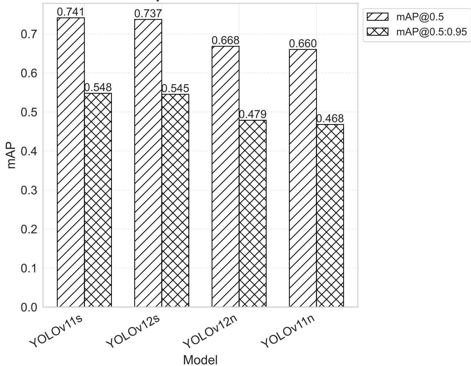
mAP Comparison Across Models
