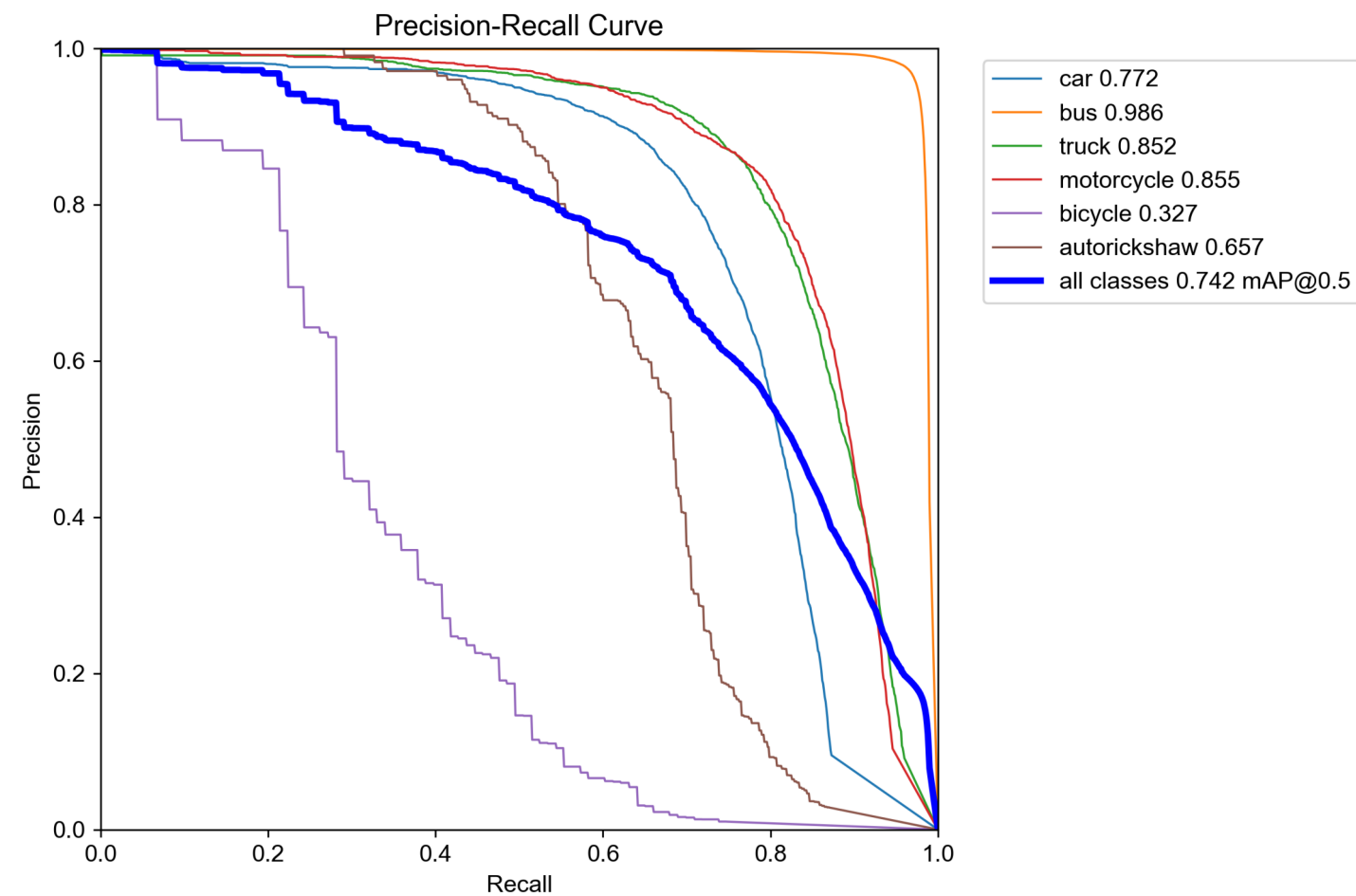
YOLOv11s
