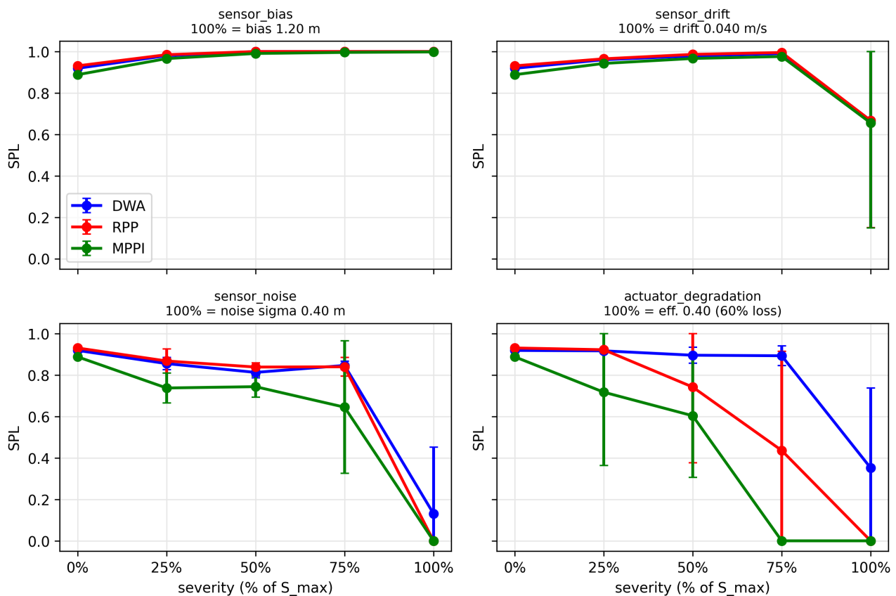
Figure 3: Dose-response SPL across fault severities. Under actuator degradation the planners separate progressively from 25% severity onward, with MPPI at zero from 75%.
