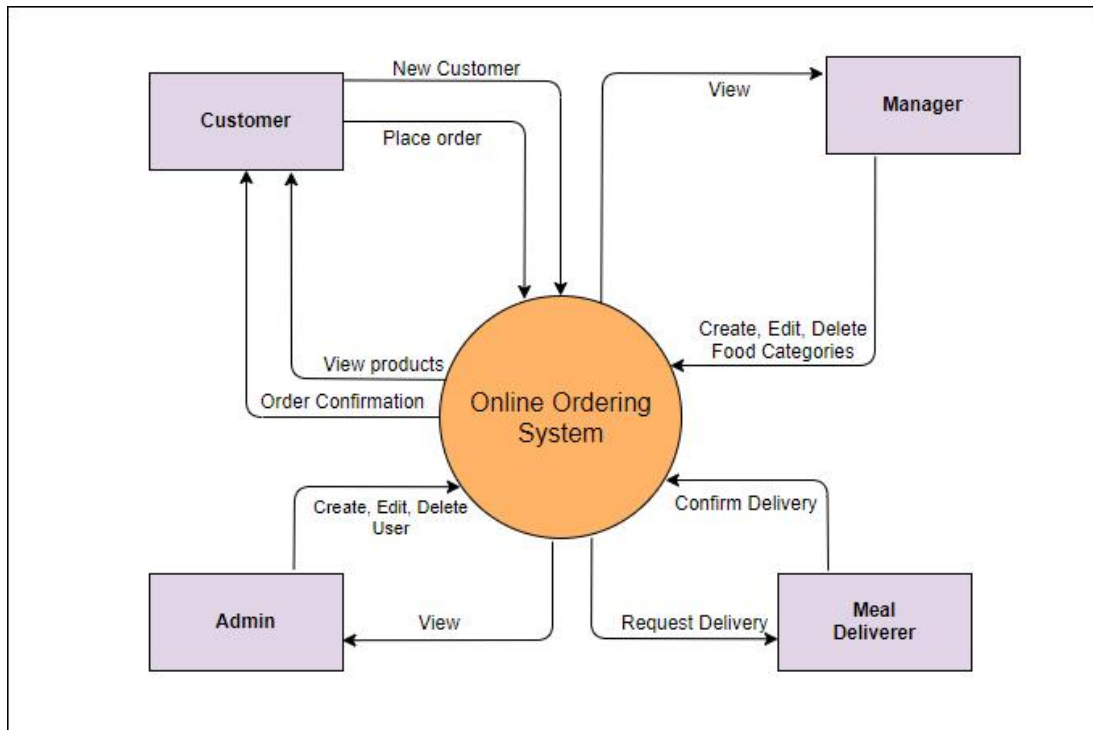
Figure 3. The Context Diagram of the Proposed Study
