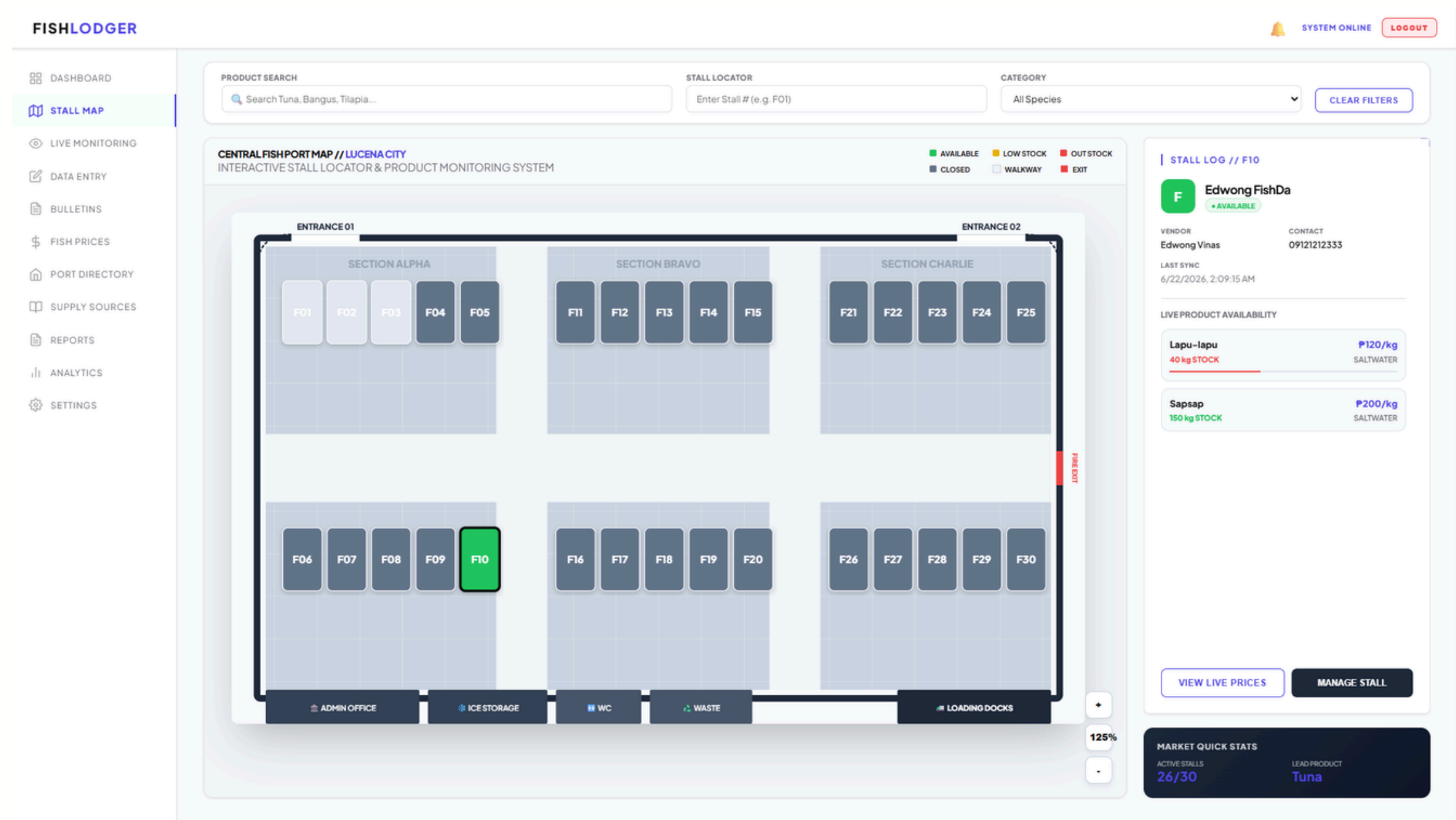
Figure 5: Stall Map
