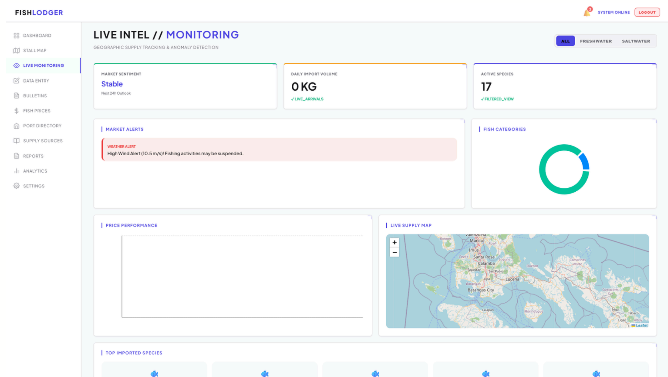
Figure 6: Live Monitoring
