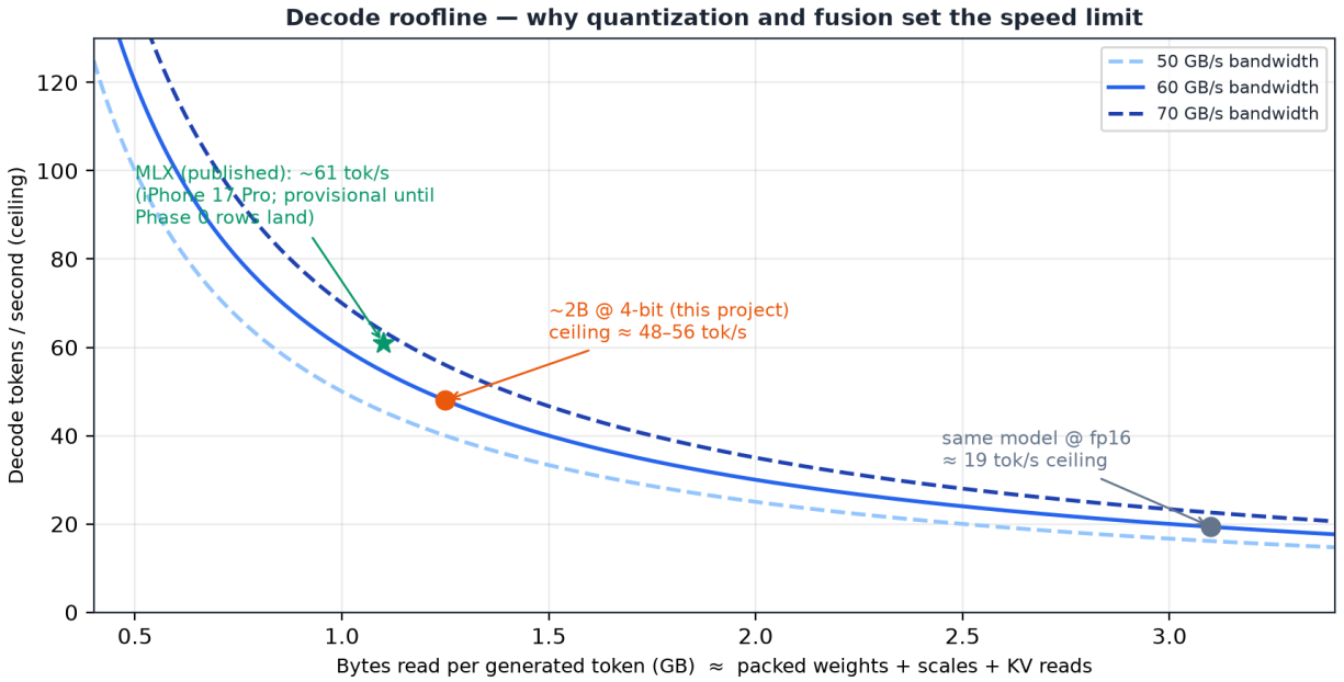
Figure 5 — Decode roofline. Curves are ceilings at three plausible bandwidths; markers show this project's operating point, the fp16 counterfactual, and MLX's published measurement.
