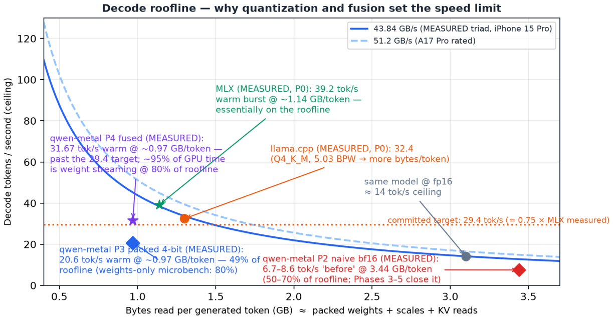
Figure 5 — Decode roofline with measured values: the 43.84 GB/s sustained triad curve, the measured MLX and llama.cpp rows, the committed 29.4 tok/s target, the fp16 counterfactual, the Phase 2 naive bf16 'before' point (6.7–8.6 tok/s, 2026-08-25), the Phase 3 packed 4-bit point (20.6 tok/s at ~0.97 GB/token, 2026-09-05), and the Phase 4 fused point (31.67 tok/s, 2026-09-14 — past the target).
