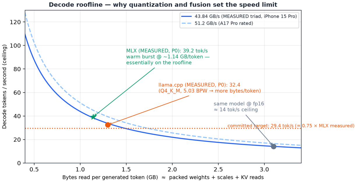
Figure 5 — Decode roofline with measured Phase 0 values: the 43.84 GB/s sustained triad curve, the measured MLX and llama.cpp rows, the committed 29.4 tok/s target, and the fp16 counterfactual.
