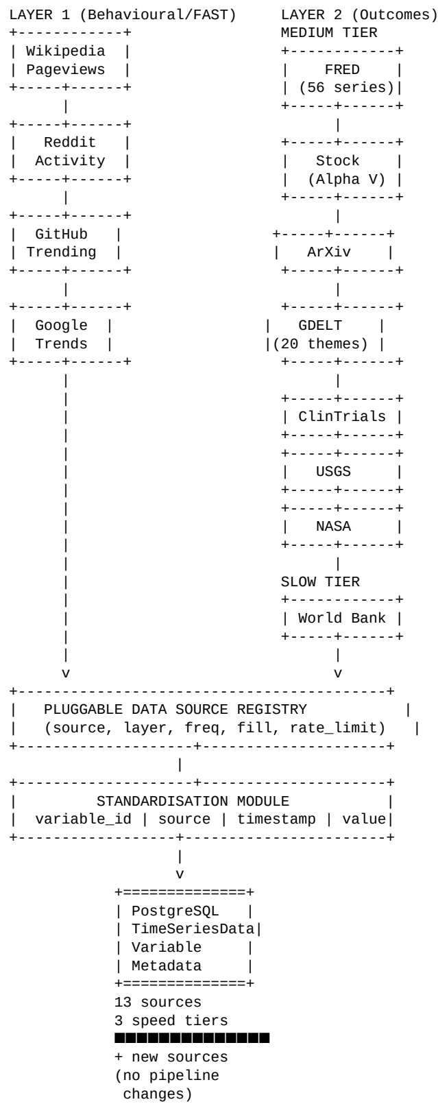
FIGURE 2: Multi-Source Data Ingestion Pipeline Innovation (1) - Variable-Level Cross-Domain Causal Discovery Claims: 1, 11, 14, 25
