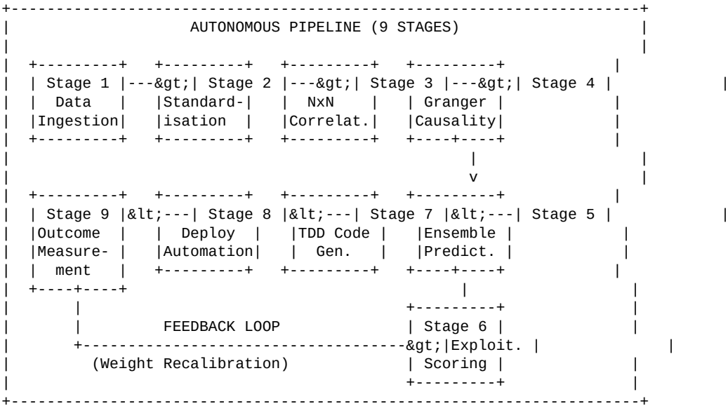
FIGURE 1: System Architecture Overview Innovation (4) - Closed-Loop Autonomous Business Pipeline Claims: 1, 14
