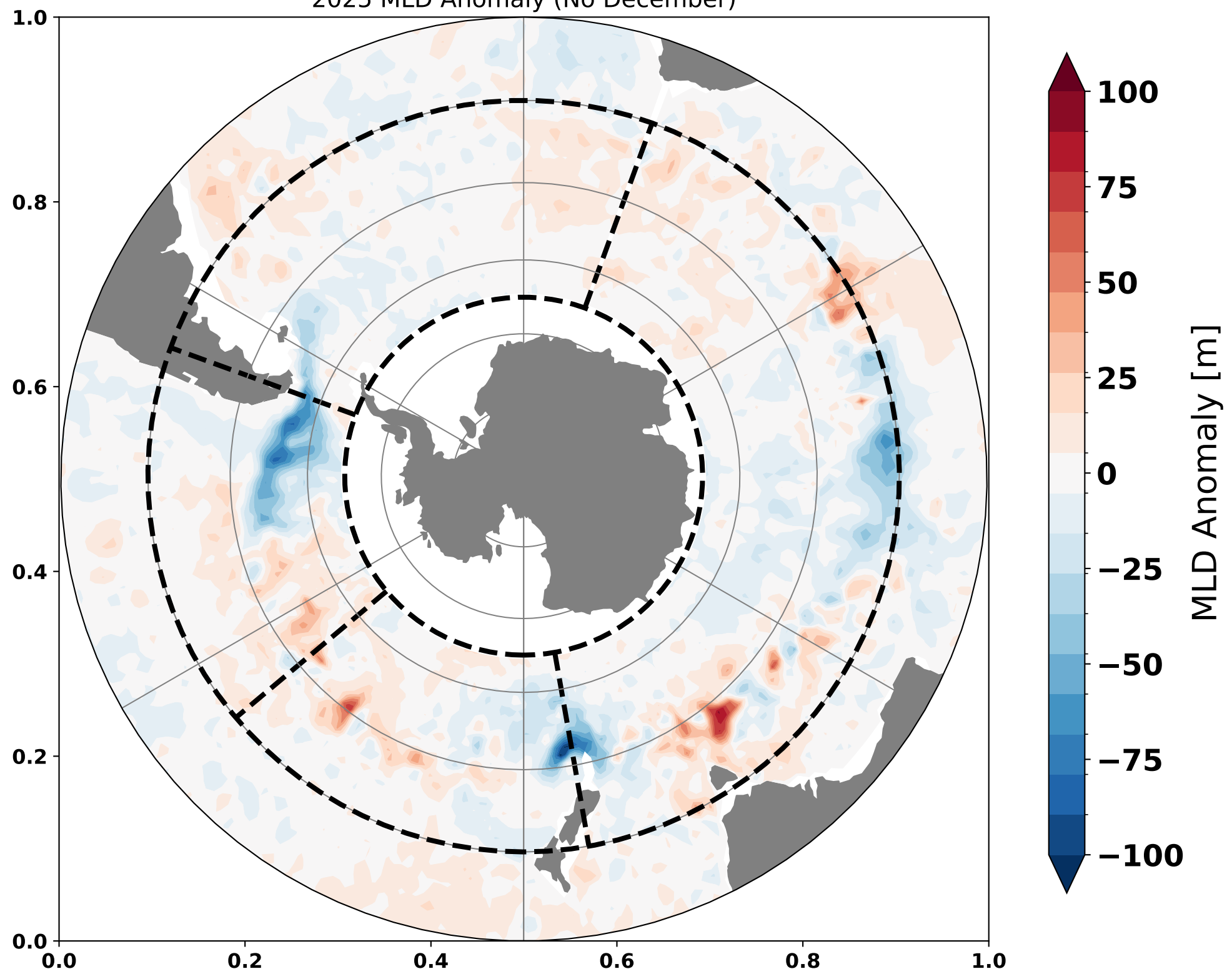
2025 MLD Anomaly (No December)
