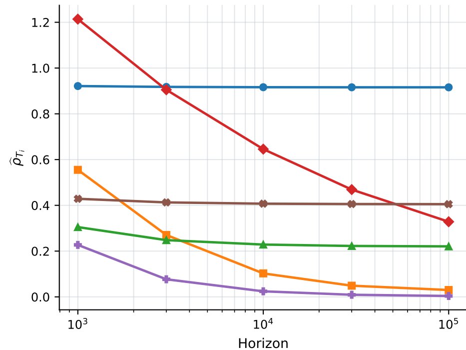
(a) Normalised regret \hat{\rho}_{T_i}
