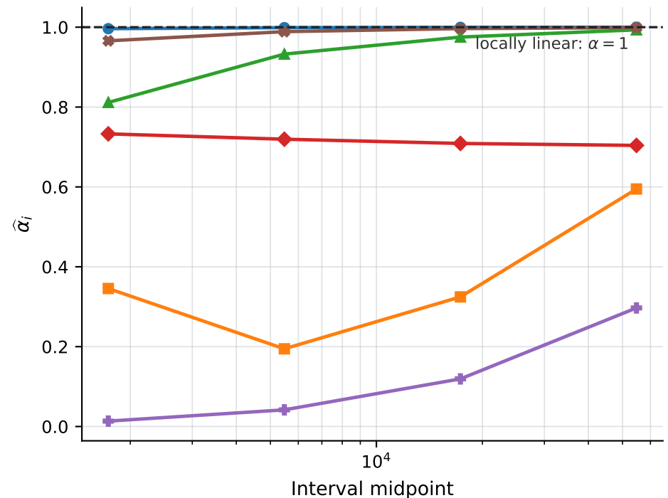
(c) Effective exponent \hat{\alpha}_i
