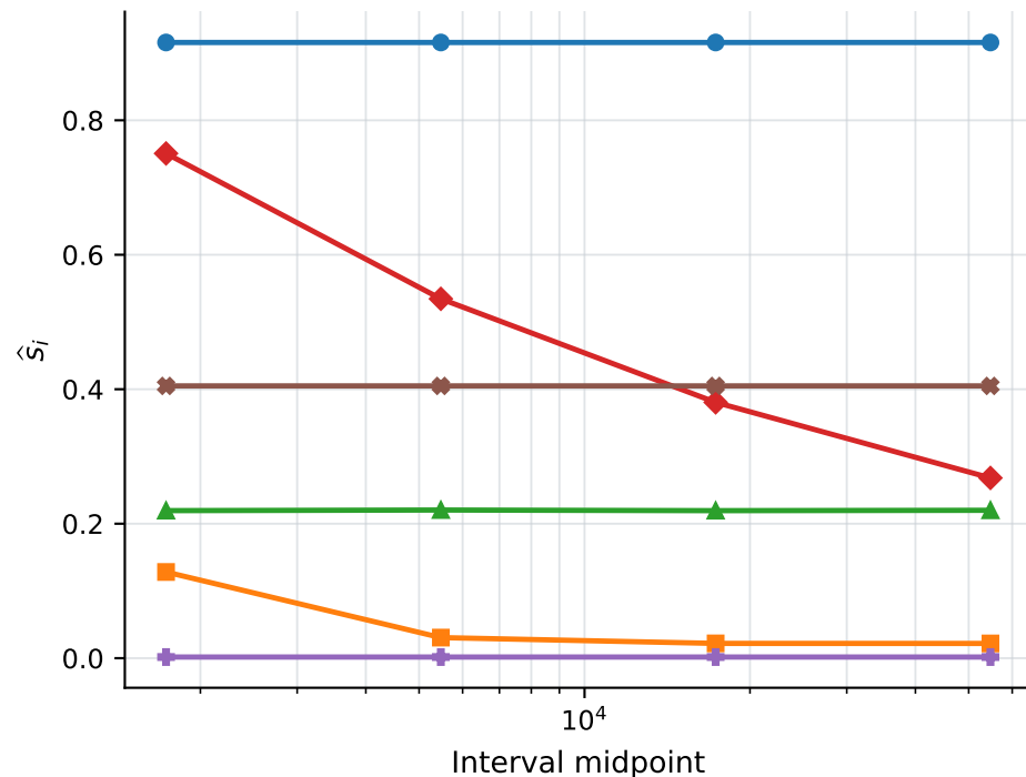
(b) Incremental rate \hat{s}_i
