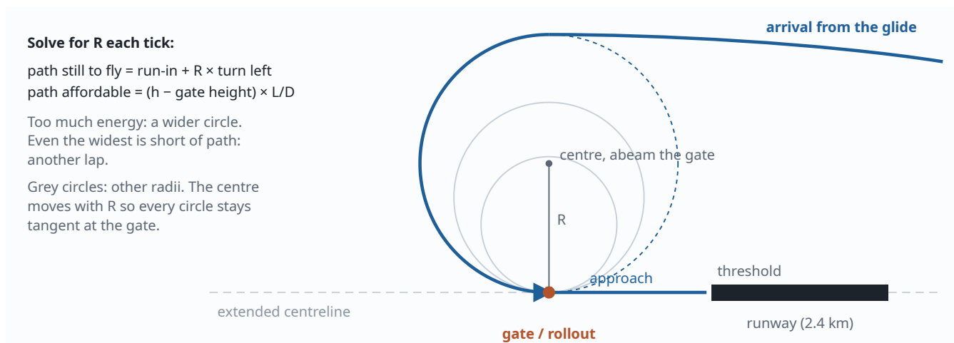
Figure 3. Plan view of the heading alignment cone. An energy error becomes a radius, and a radius is something the vehicle can just fly. The circle is entered only below Mach 1.5: turn radius goes as v^2 , about 9 km at Mach 0.9 and 250 km at Mach 4.7.
