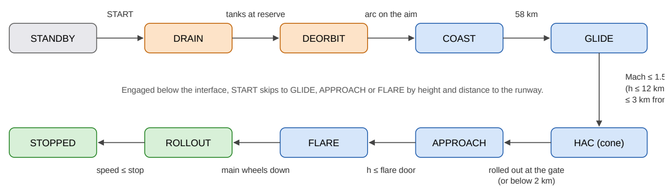
Figure 1. Phases and the conditions that advance them. Orange phases use the engine; blue are unpowered flight; green is on the ground.
