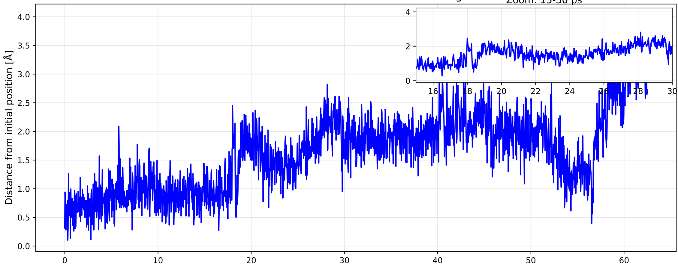
Water Molecule 133: Relative to Initial Configuration Zoom: 15-30 ps
