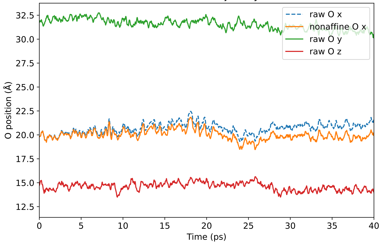
Particle 34 trajectory
