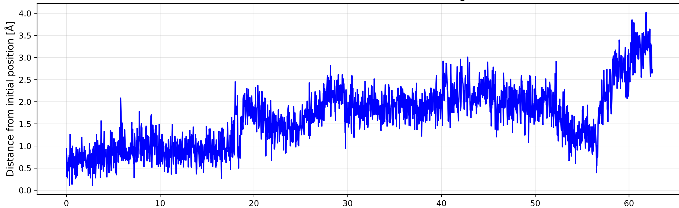
Water Molecule 133: Relative to Initial Configuration
