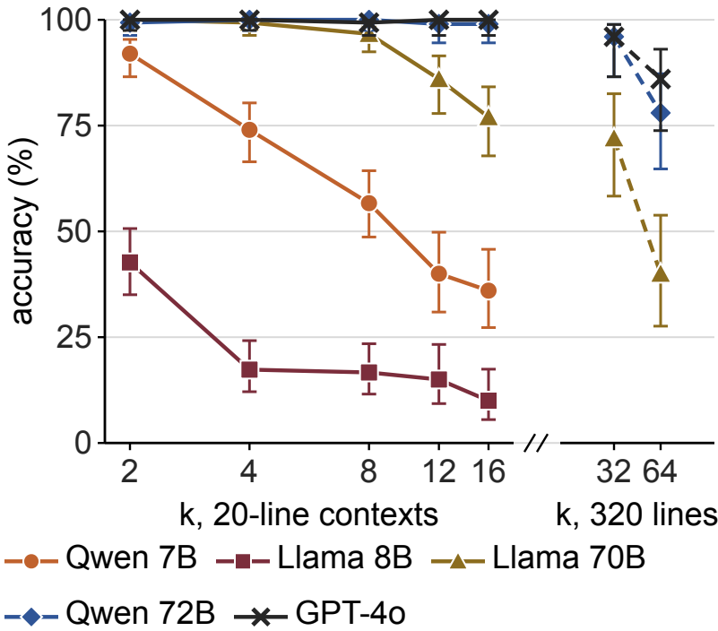
(b) Scaling with direct answers accuracy; bars: 95% intervals
