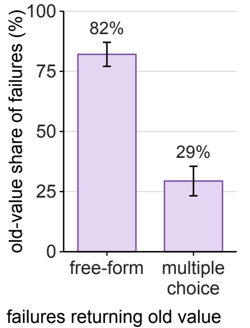
(c) Multiple choice hides it ICF-Bench; acc. 69 vs. 71%
