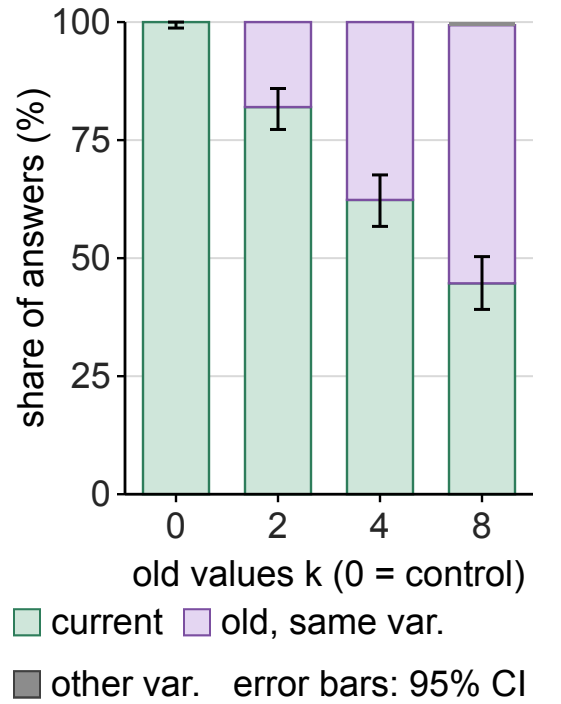
(a) What the model answers 300 per column, all lengths pooled
