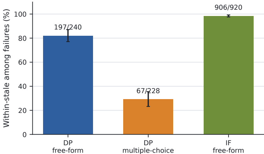
Multiple-choice masks stale-binding
