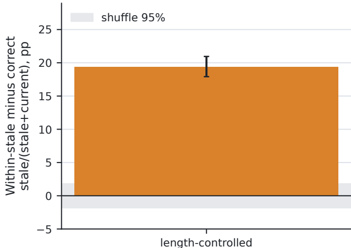
Stale-attention signature
