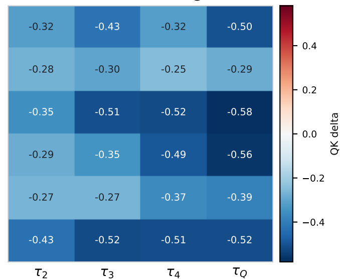
QK selection margin
