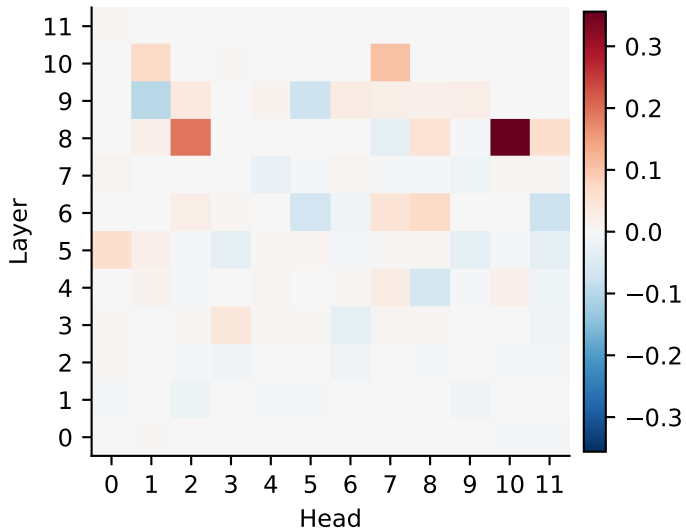
b Clean-to-corrupt head-patch recovery
