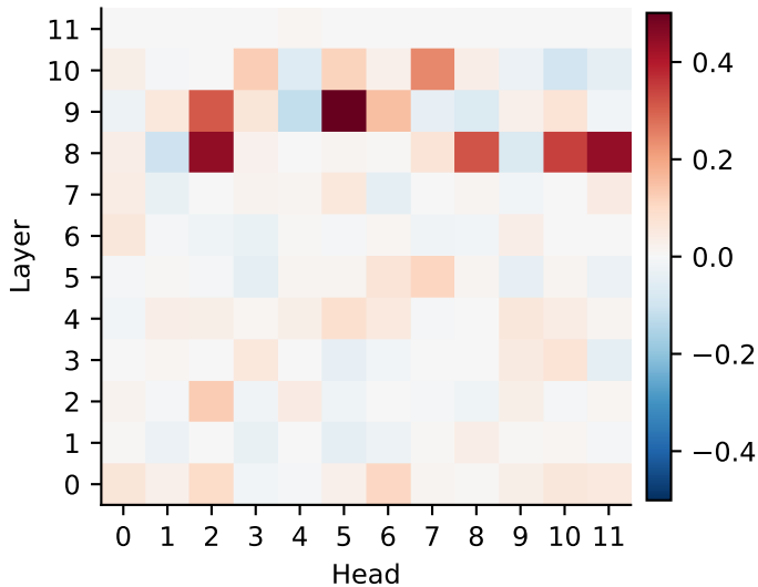
a Stale-attention shift (length controlled)
