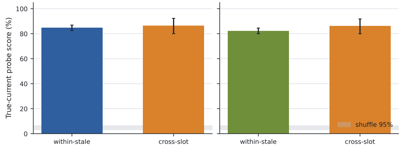
Qwen2.5-7B
