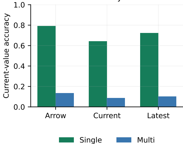
b Format sensitivity at fixed k=4
