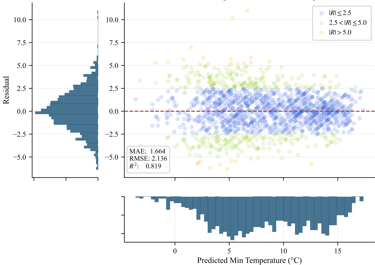
TCN + CTGAN (processed) – Seattle / Temp Min
