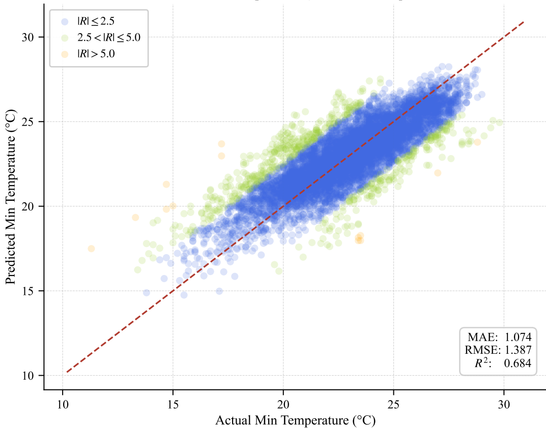
TCN + CTGAN (processed) – Seoul / Temp Min
