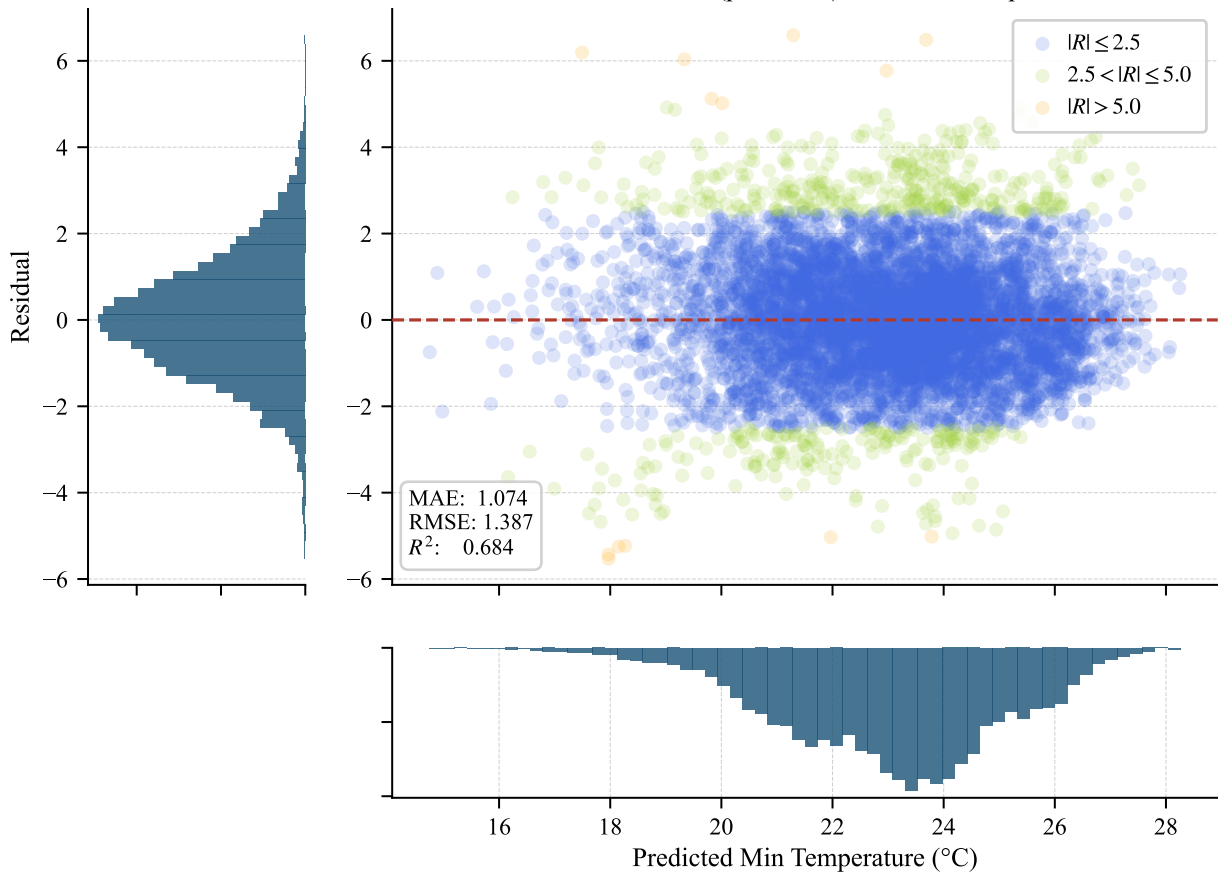
TCN + CTGAN (processed) – Seoul / Temp Min
