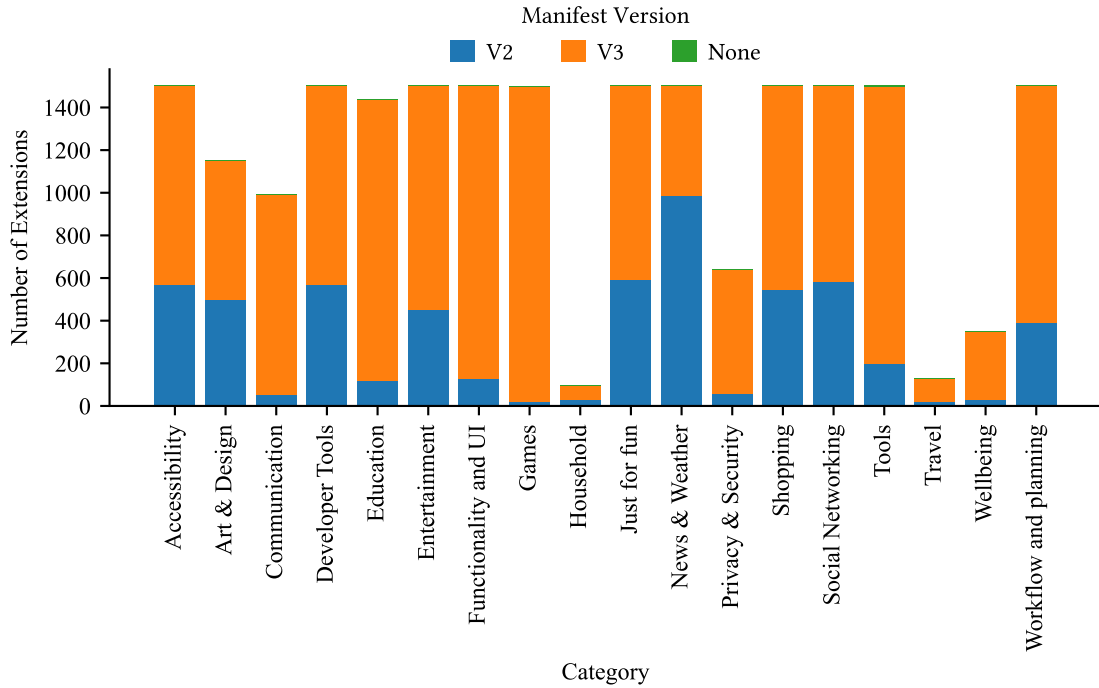
Figure 3: Manifest Version of Extensions per Category
