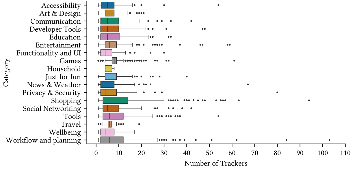
Figure 13: Boxplot of the Number of Trackers for the WordPress Blog HoneyPage.
