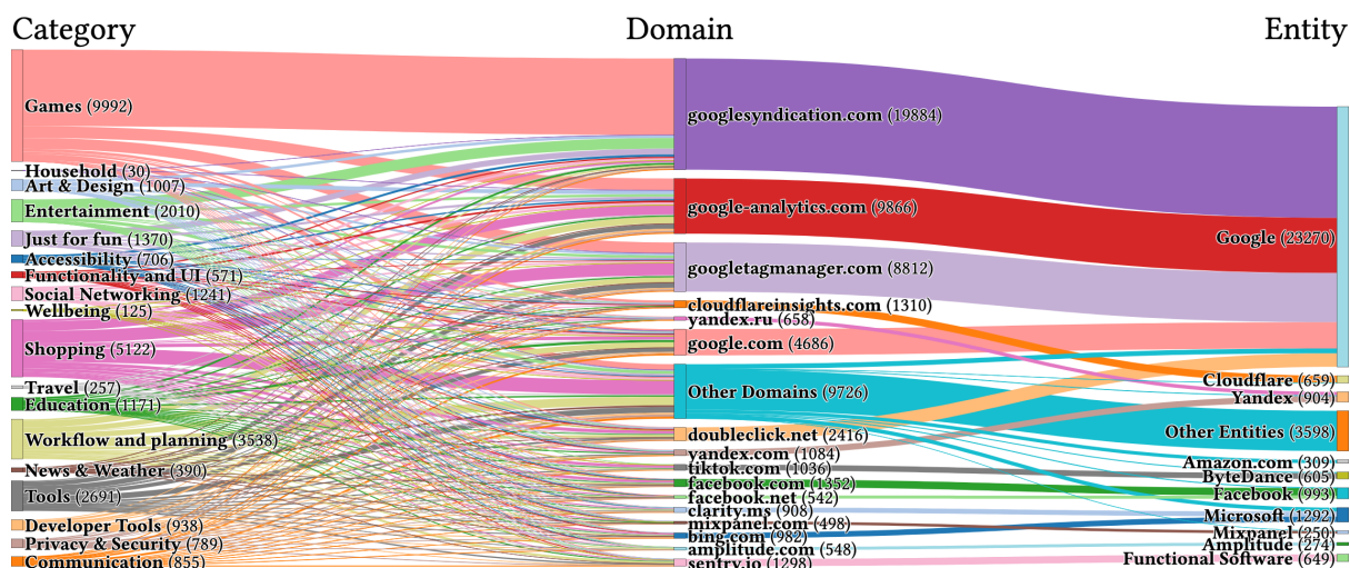
Figure 10: Mapping of Trackers, from Extension Categories to Domains to Domain Owner for the WordPress 404 HoneyPage. (Other is less than 400.)
