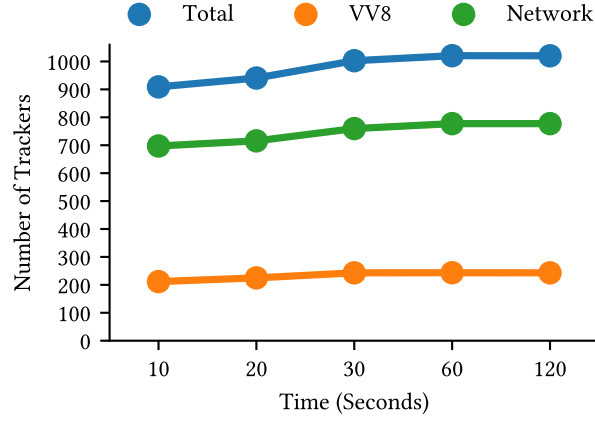
Figure 2: Results of Crawl Time Experiments
