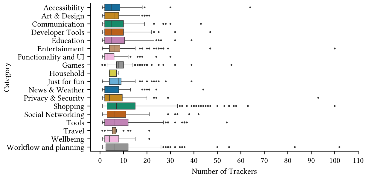
Figure 11: Boxplot of the Number of Trackers for the WordPress Index HoneyPage.
