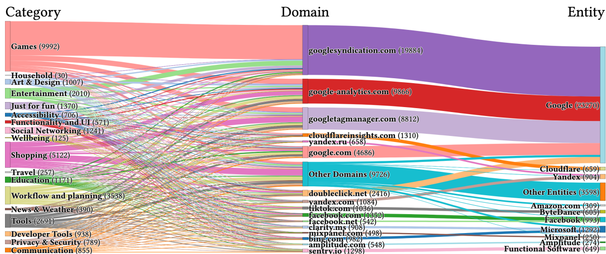
Figure 9: Mapping of Trackers, from Extension Categories to Domains to Domain Owner for the WordPress Blog HoneyPage. (Other is less than 400.)
