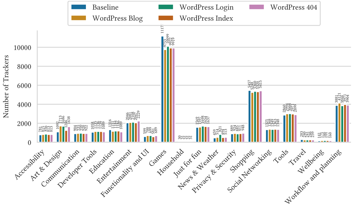
Figure 6: Number of Trackers per Category over HoneyPages
