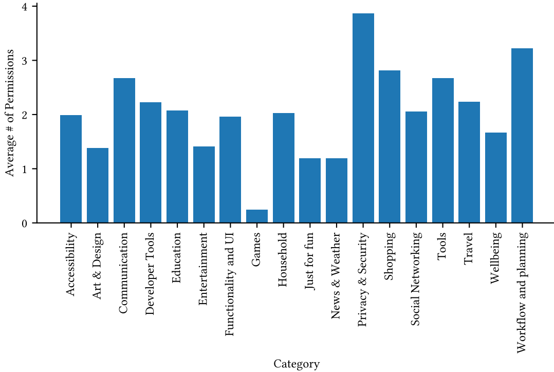
Figure 4: Average Number of Permissions of Extensions per Category
