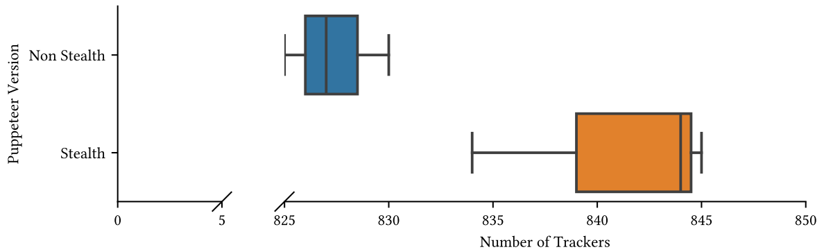
Figure 1: Box plots of the Number of Trackers for Puppeteer and Puppeteer Stealth.
