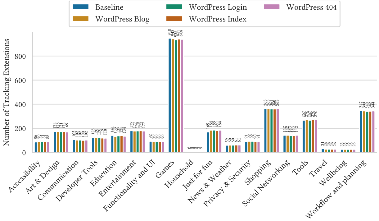
Figure 5: Number of Tracking Extensions per Category over HoneyPages
