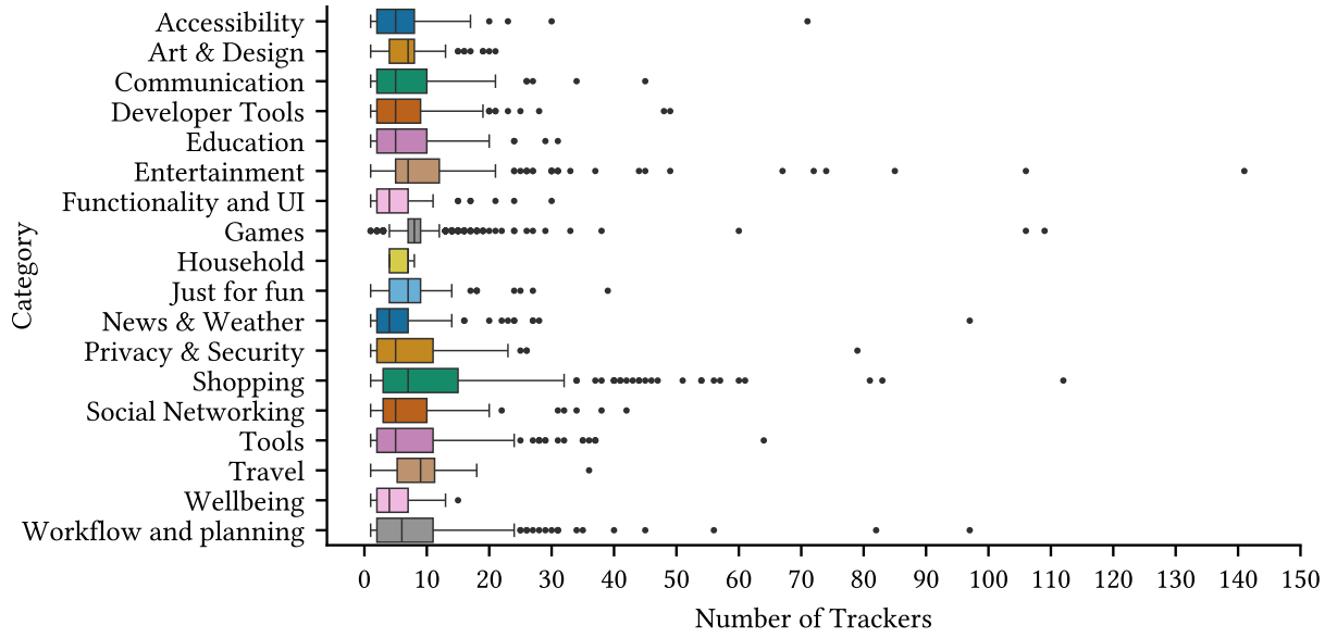
Figure 14: Boxplot of the Number of Trackers for the WordPress 404 HoneyPage.
