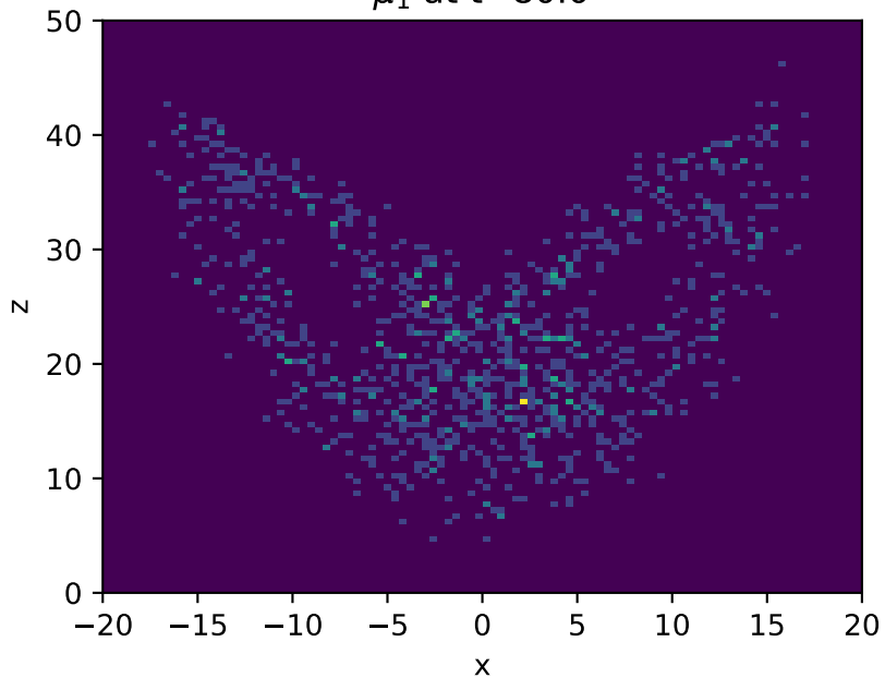
\mu_1 at t=80.0
