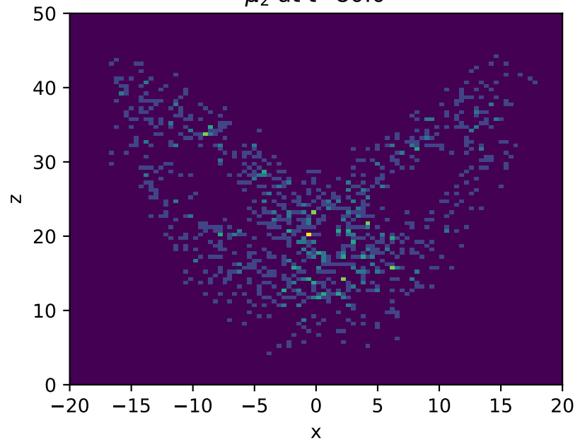
\mu_2 at t=80.0
