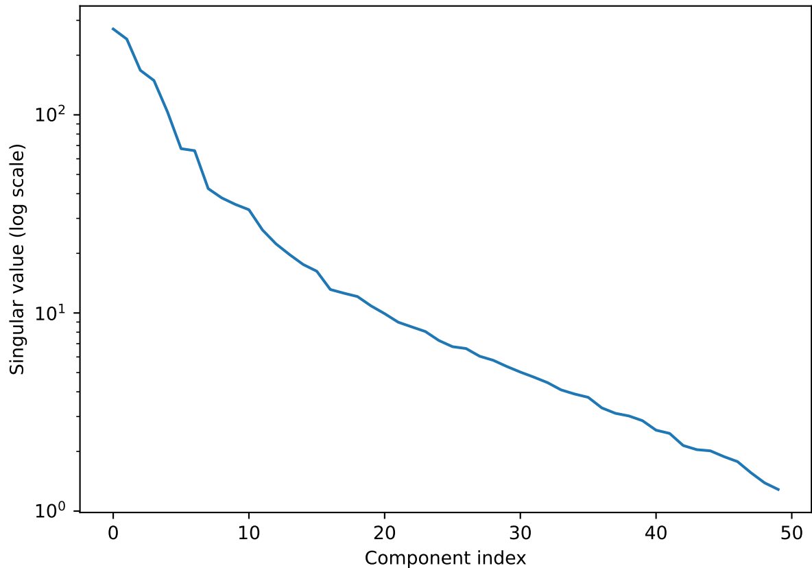
Singular Value Decay
