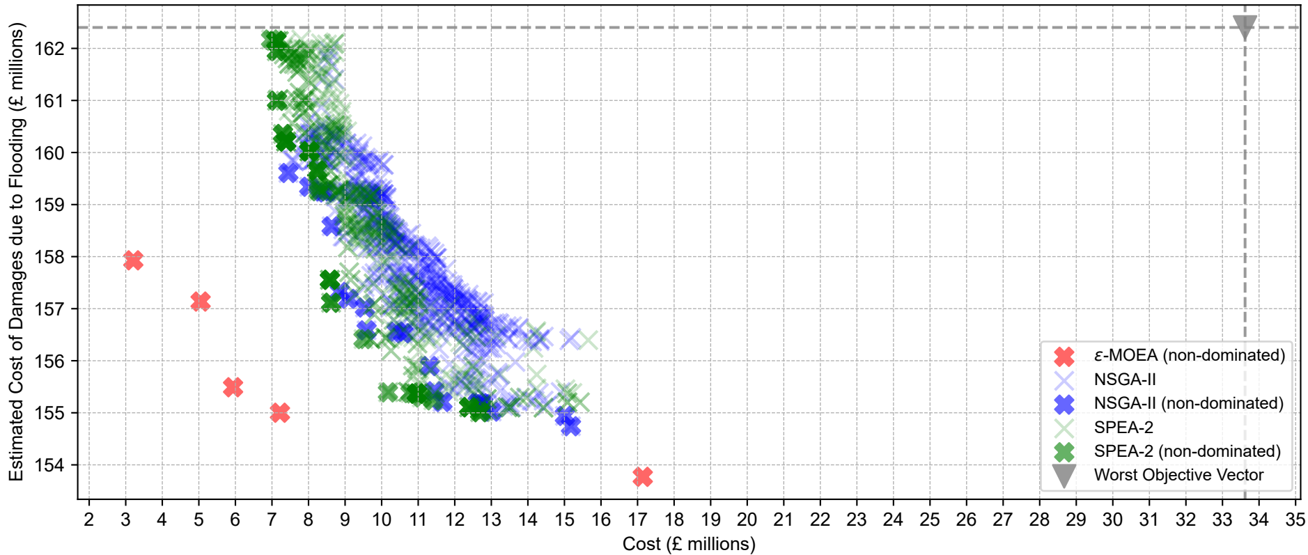
Final Solutions \epsilon -MOEA simulations = 1049, NSGA-II simulations = 3032, SPEA-2 simulations = 3025
