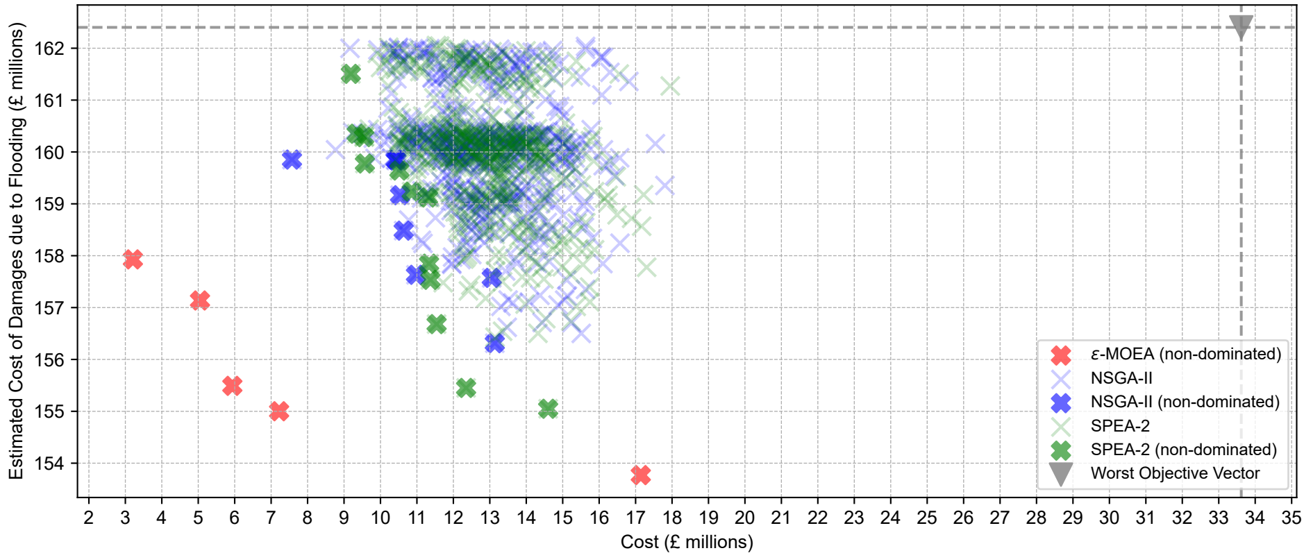
Final Solutions \epsilon -MOEA simulations = 1049, NSGA-II simulations = 1012, SPEA-2 simulations = 1012
