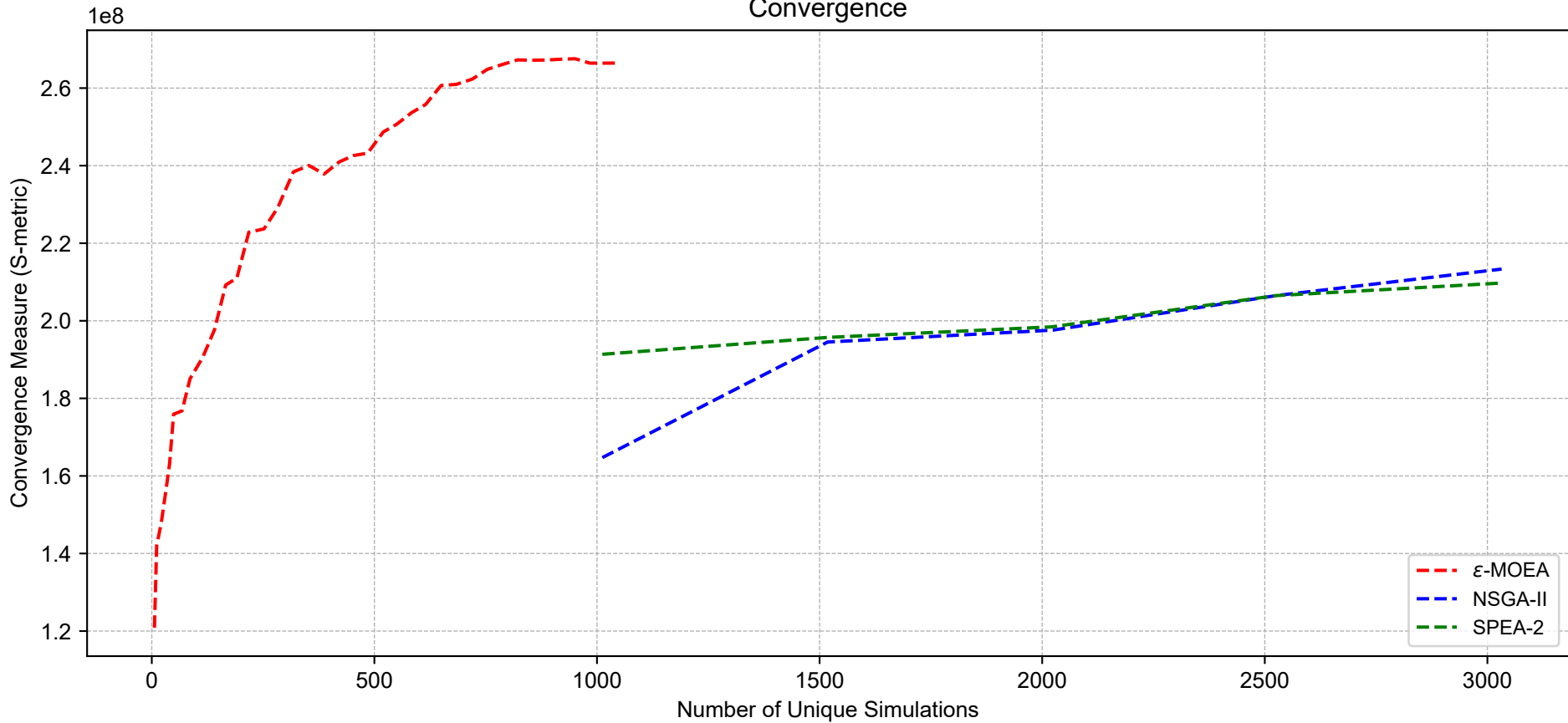
Convergence
