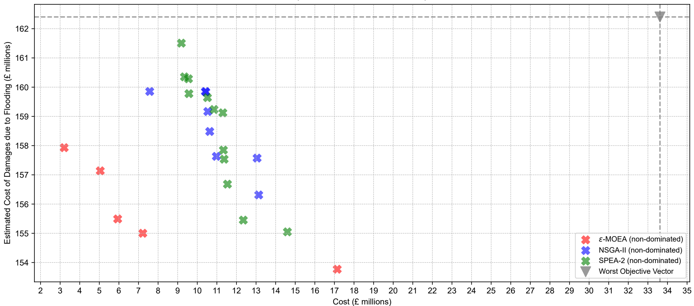
Final Solutions \epsilon -MOEA simulations = 1049, NSGA-II simulations = 3032, SPEA-2 simulations = 3025
