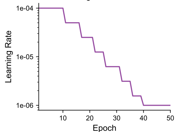
Learning Rate Schedule
